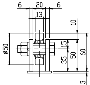
端部断面詳細 (1/2.5)
